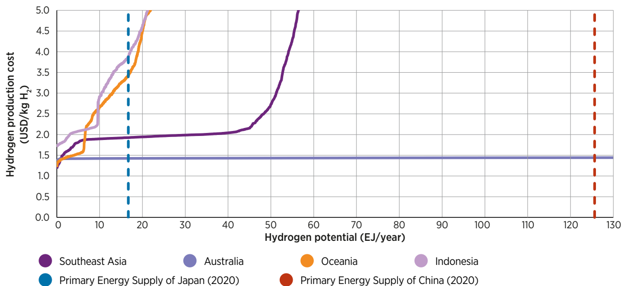
Figure 64 Hydrogen cost curve potential based on 2030 values
