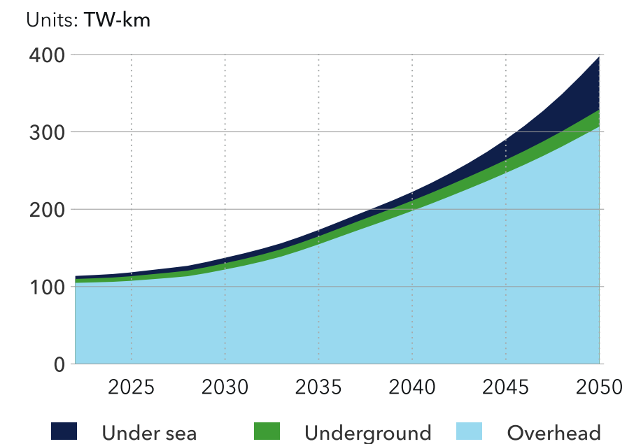
FIGURE 2.12 HVDC grid capacity by power-line type
