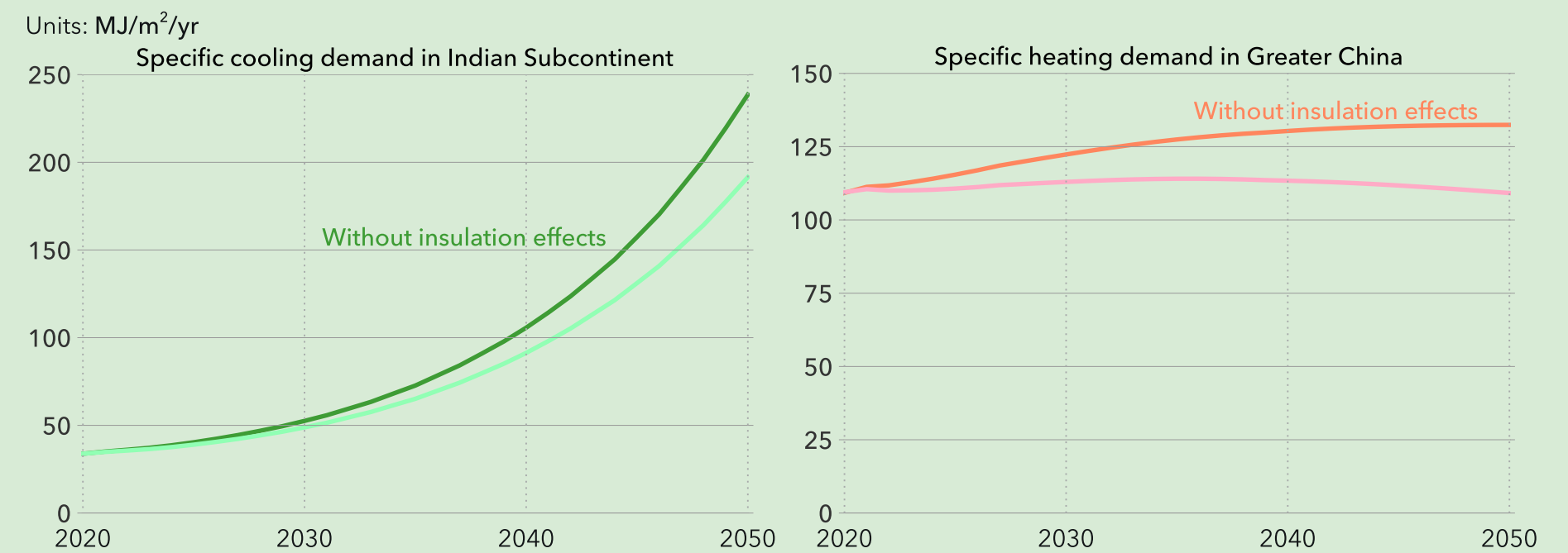
FIGURE 1.21 Effect of insulation on specific space heating and cooling demand
