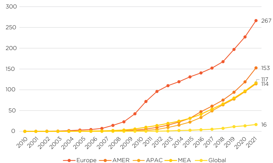
Fig 26. Watt per capita solar PV by region, 2000-2021
