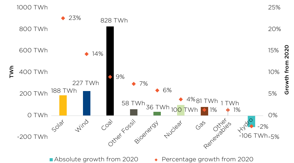
Fig 46. Power technologies used to meet global additional electricity demand in 2021
