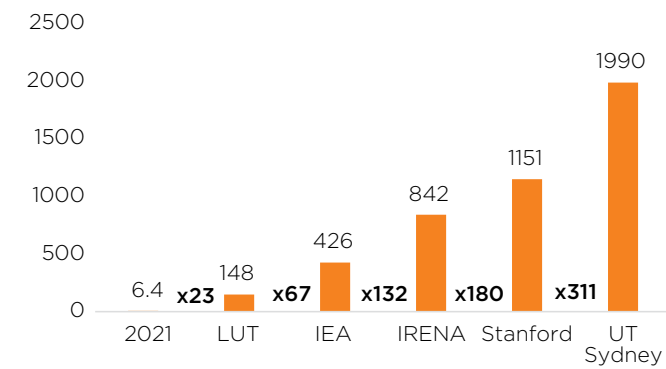
Fig 70. CSP - Total installed capacity scenarios 2050
