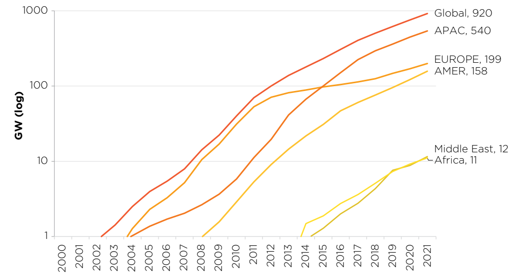
Fig 12. Cumulative solar PV deployment by region, 2000-2021
