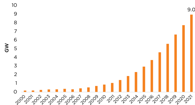
Fig 35. Cumulative off-grid solar PV capacity 2000-2021
