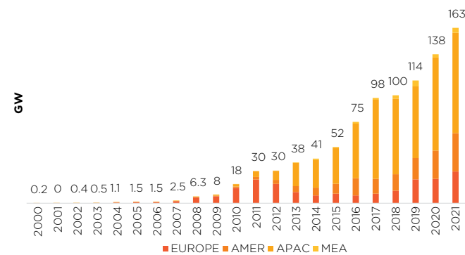
Fig 8. Annual global solar PV deployment, 2000-2021
