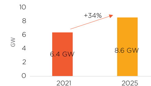
Fig 62b. CSP - Total installed capacity 2021 and 2025
