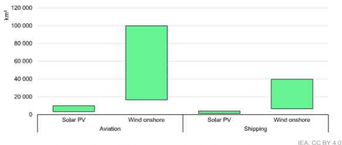
Figure 6.7 Total land needs for achieving a 10% share of low-emission e-fuels in 2030 by transport sector
