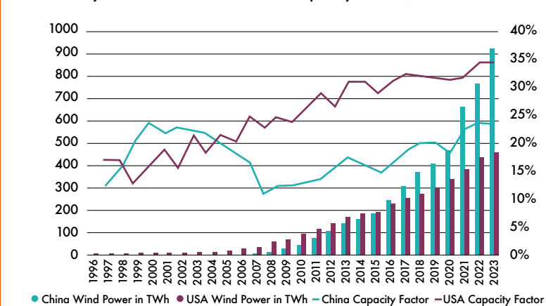
Wind Yearly Generation in TWh and Capacity Factor, China vs US
